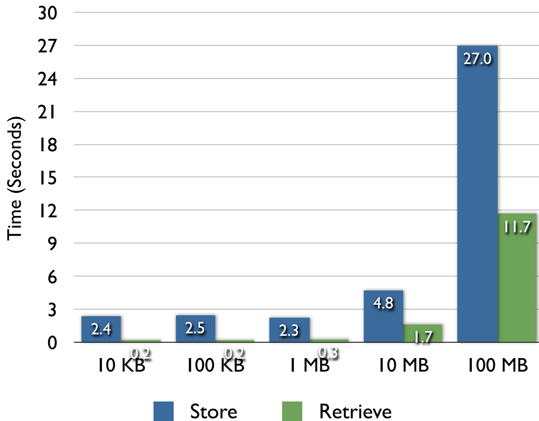
Mimir Performance
