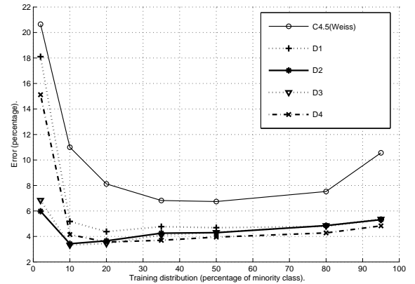
Fig. 6. Wisconsin: the error in classification over various degrees of class distributions. Natural distribution is 35%.
