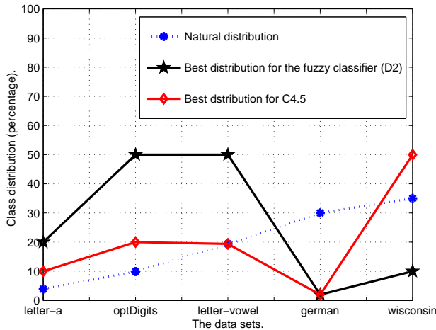
Fig. 12. The best distribution for learning versus natural distribution.
