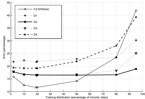
Fig. 4. Letter-vowel: the error in classification over various degrees of class distributions. Natural distribution is 19.4%.
