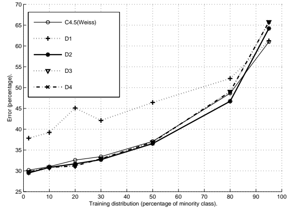
Fig. 5. German: the error in classification over various degrees of class distributions. Natural distribution is 30%.
